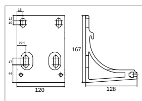
SUPPORT POSE DE FACE LARGE
