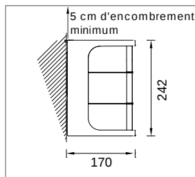
SUPPORT POSE DE FACE LARGE
