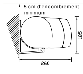
SUPPORT POSE DE FACE LARGE
