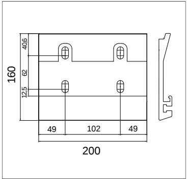
SUPPORT 200 MM
