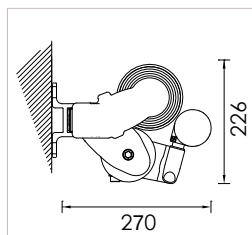
SUPPORT FACE
