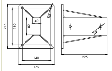
PIED PLATINE 175x215
