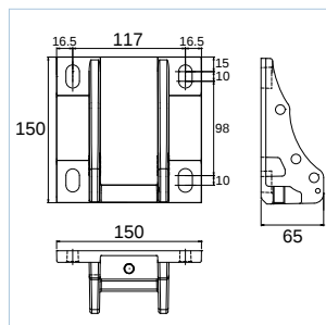
SUPPORT POSE DE FACE
