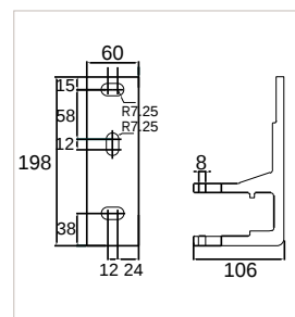
SUPPORT POSE DE FACE
