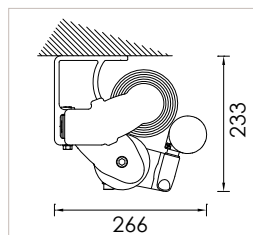
SUPPORT PLAFOND
