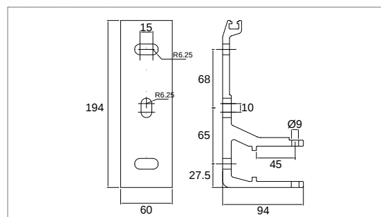
SUPPORT POSE DE FACE
