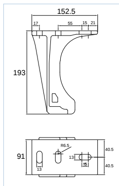
SUPPORT PLAFOND
