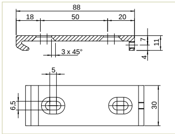
SUPPORT FIXATION COFFRE
