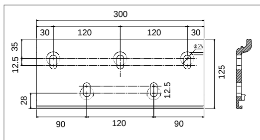
SUPPORT POSE DE FACE LARGE DE SÉRIE
