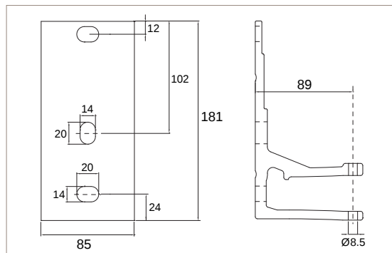
SUPPORT POSE PLAFOND
