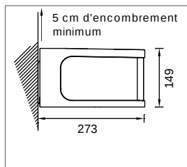
SUPPORT POSE DE FACE LARGE DE SÉRIE
