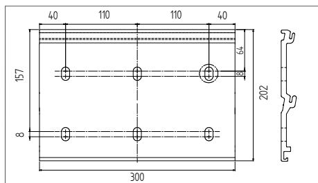
SUPPORT POSE DE FACE LARGE
