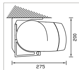
EQUERRE POSE PLAFOND LARGE
