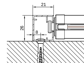
Coulisse pose murale
