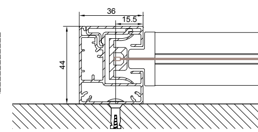
Coulisse pose murale
