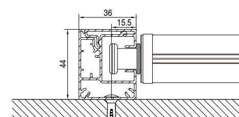
Coulisse pose murale
