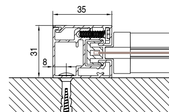
Coulisse pose murale
