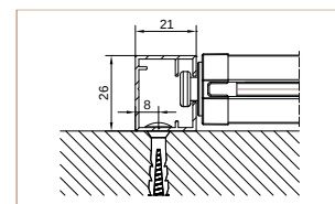
COULISSE POSE MURALE
